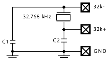
Figure 5. 32.768 kHz Oscillator
