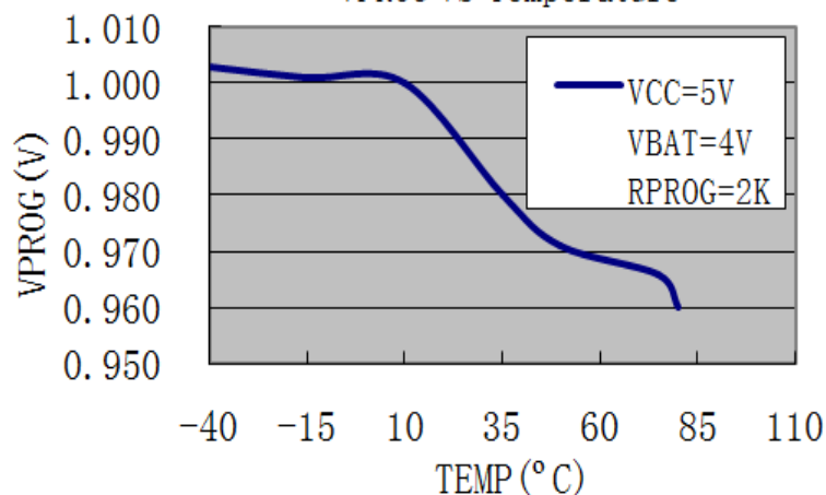
VPROG VS Temperature
