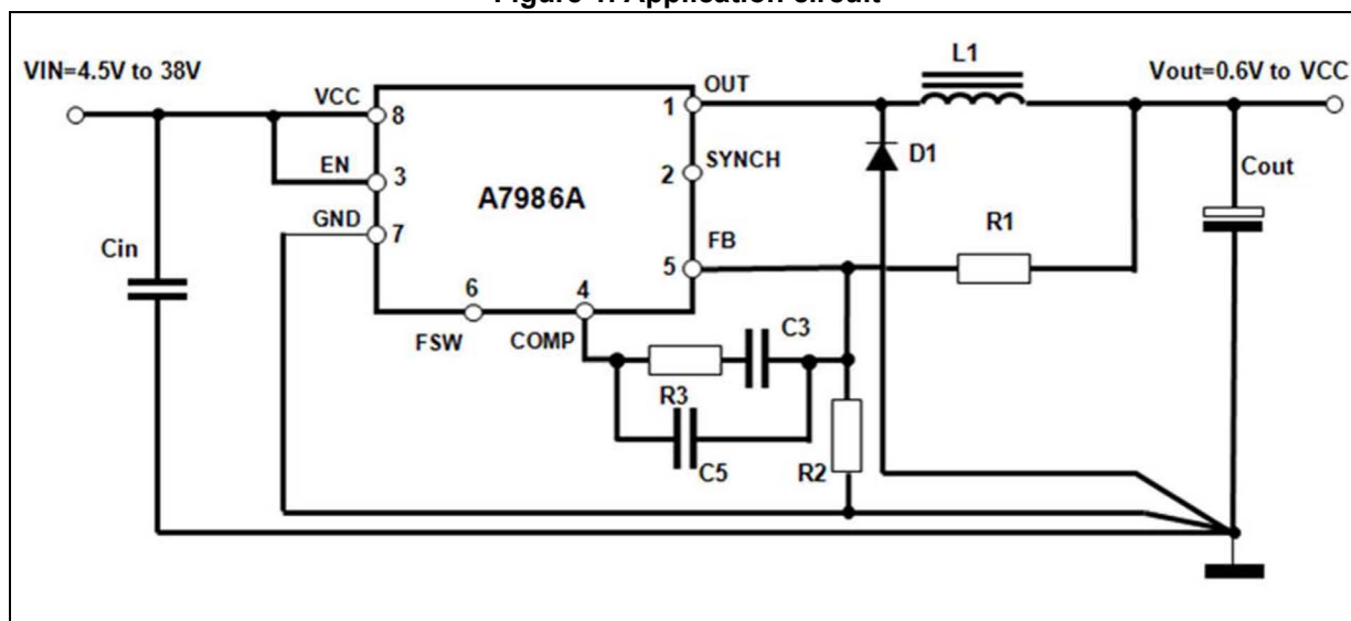
Figure 1. Application circuit
