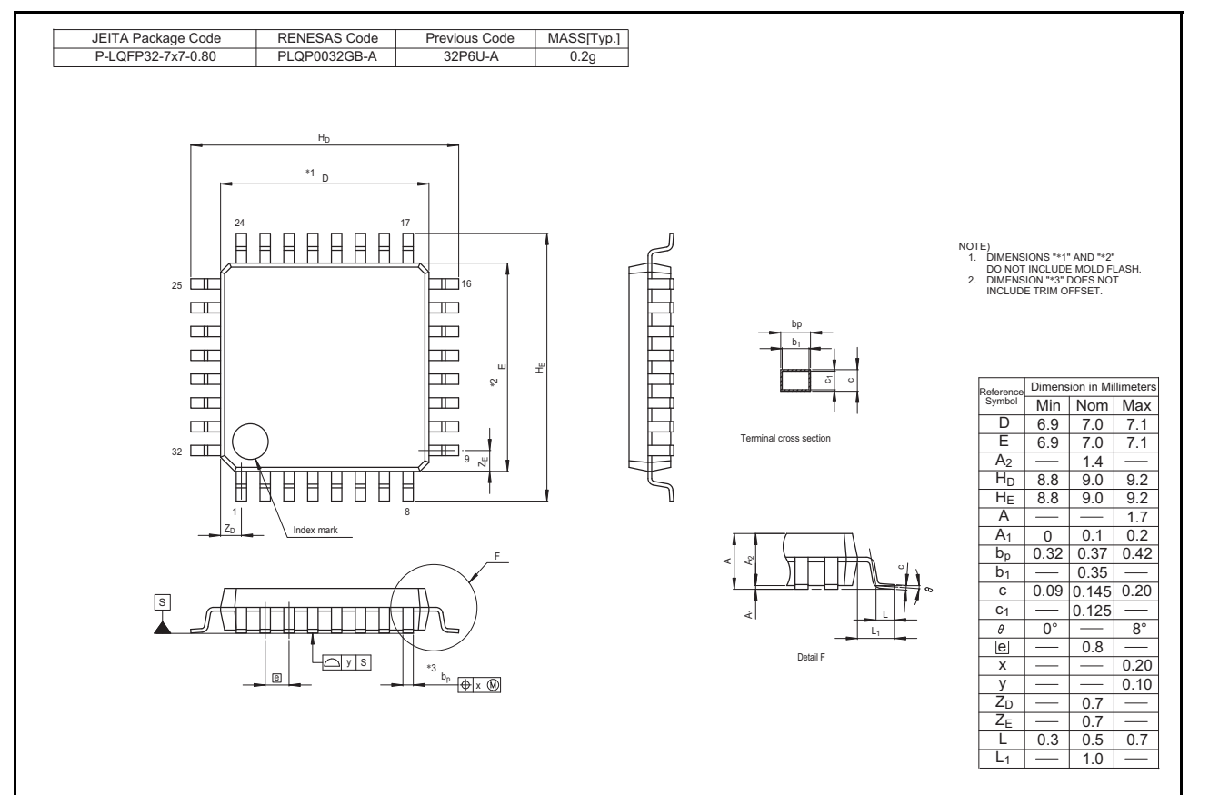
Figure 1.2 LQFP 32-pin
