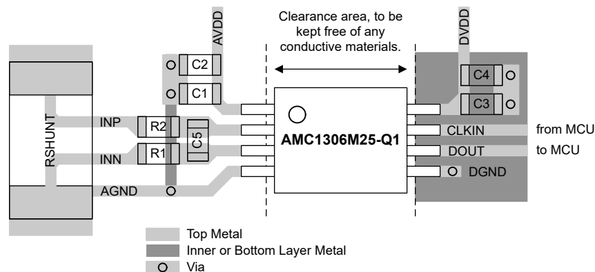
Figure 10-1. Recommended Layout of the AMC1306M25-Q1
