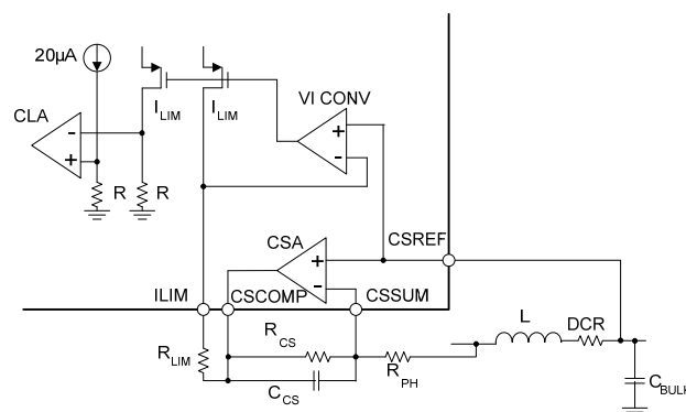
Figure 28. Current Limit Circuit
