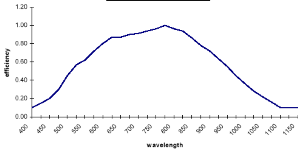
Monochrome Response
