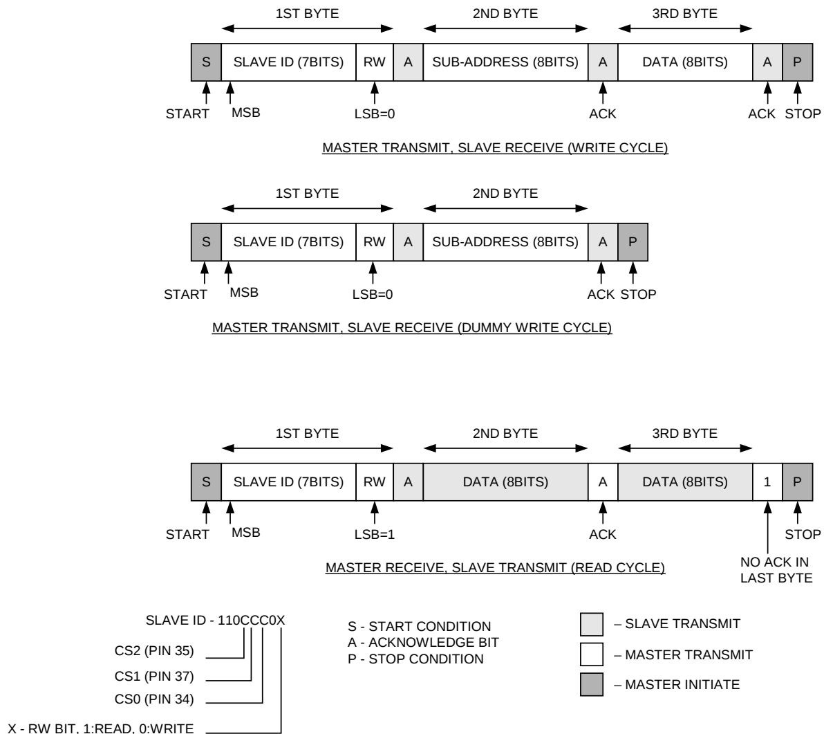
Figure 8. I 2 C Bus Protocol Format
