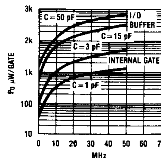
FIGURE 2. Power Consumption vs Frequency
