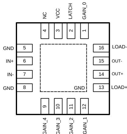
Figure 1. 16-Pin WQFN (Top View)
