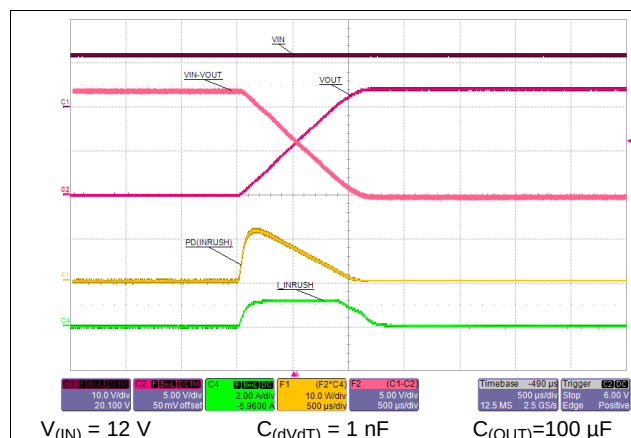
Figure 53. Start-up Without Load
