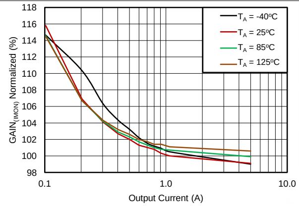
Figure 24. \text{GAIN}_{(IMON)}\% Normalized vs Output Current
