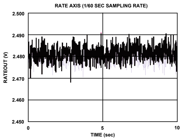
Figure 12. 10 g Random Vibration in Rate Axis Orientation
