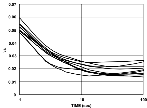
Figure 8. Root Allan Variance vs. Averaging Time
