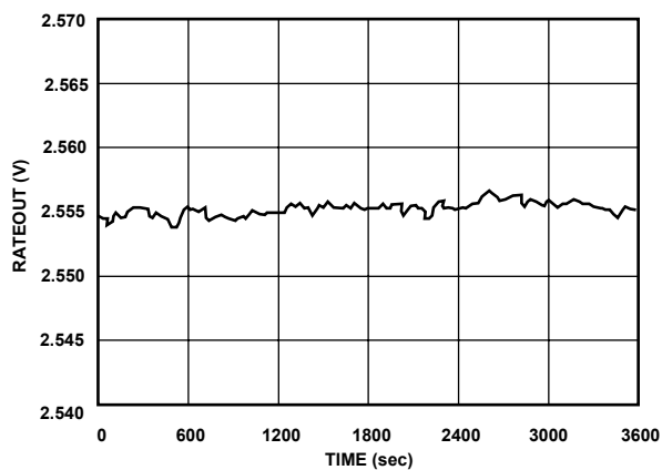
Figure 5. Null Stability for 1 Hour
