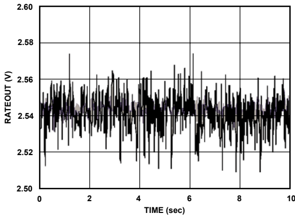
Figure 24. Random Vibration (Lateral) 10 kHz to 20 kHz at 0.01 g/\sqrt{\text{Hz}} with 60 Hz Sampling and 0.5 sec Averaging
