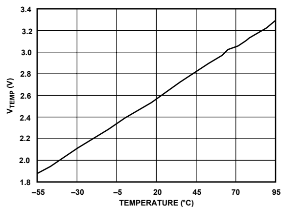
Figure 6. Temperature Sensor Output
