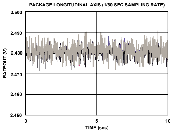
Figure 11. 10 g Random Vibration in Package-Longitudinal Axis Orientation
