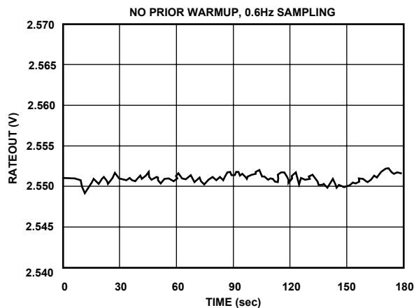
Figure 7. Null Settling Time
