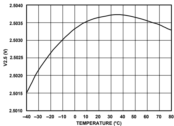
Figure 9. 2.5 V Voltage Reference vs. Temperature
