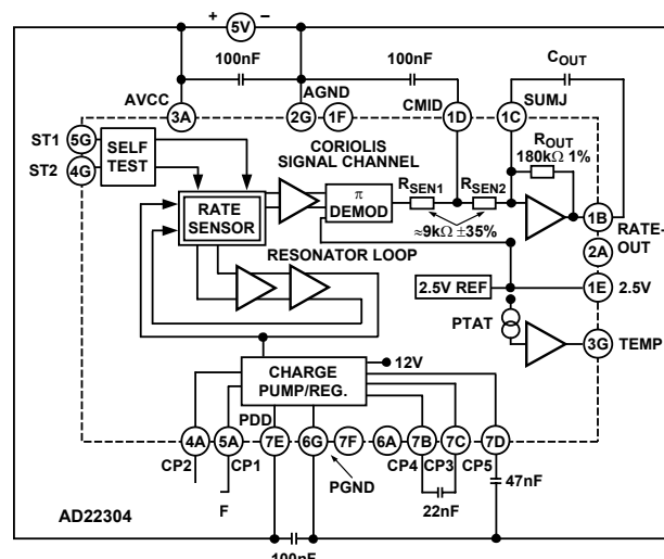
Figure 23. Block Diagram with External Components
