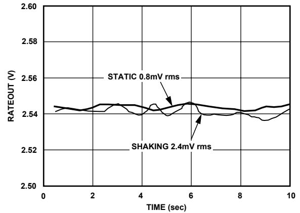
Figure 26. Random Vibration (Lateral) 10 kHz to 20 kHz at 0.01 g/\sqrt{\text{Hz}} with 60 Hz Sampling and 0.5 sec Averaging
