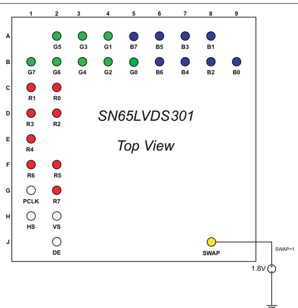
Figure 8-3. SWAP PIN = 1
