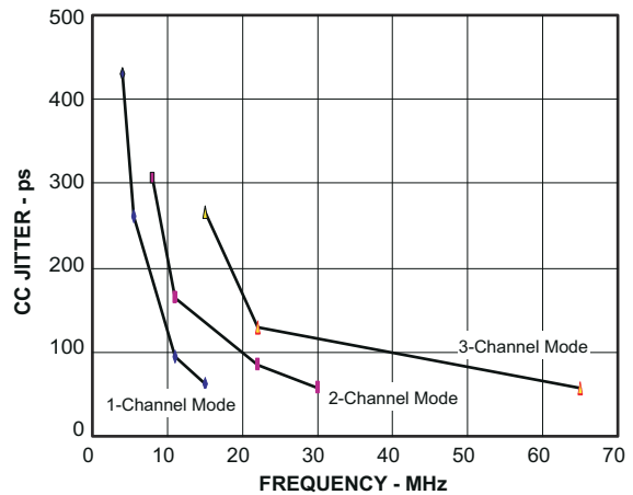
Figure 6-7. Cycle-to-cycle Output Jitter vs PCLK Frequency
