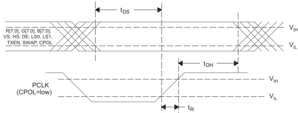
Figure 7-1. Setup/Hold Time
