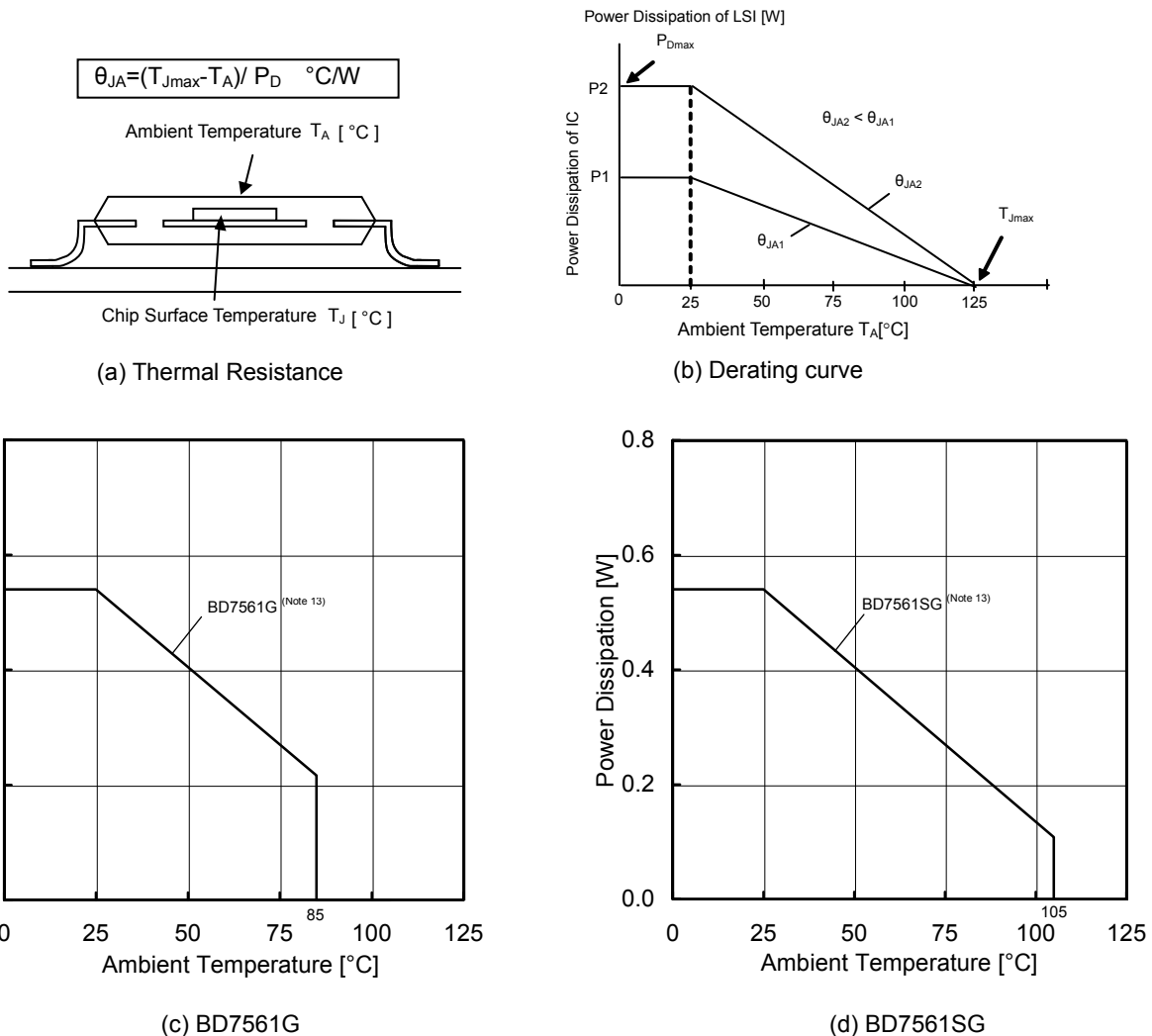
Figure 52. Thermal Resistance and Derating Curve
