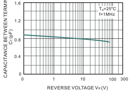
Fig.4 Capacitance Characteristics
