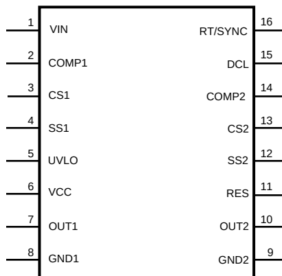
PW Package 16-Pin TSSOP Top View
