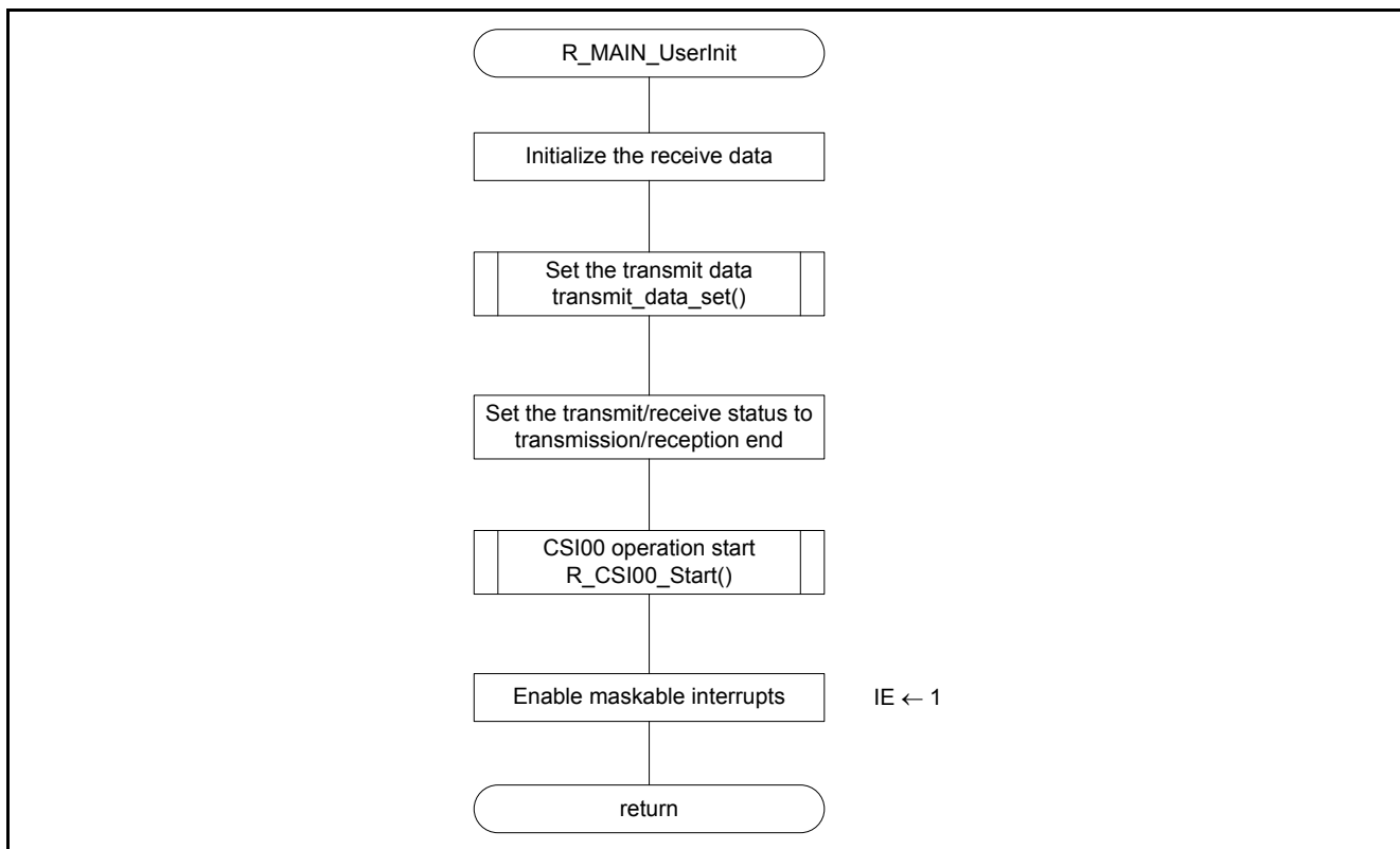
Figure 4.20 Main Initialization
