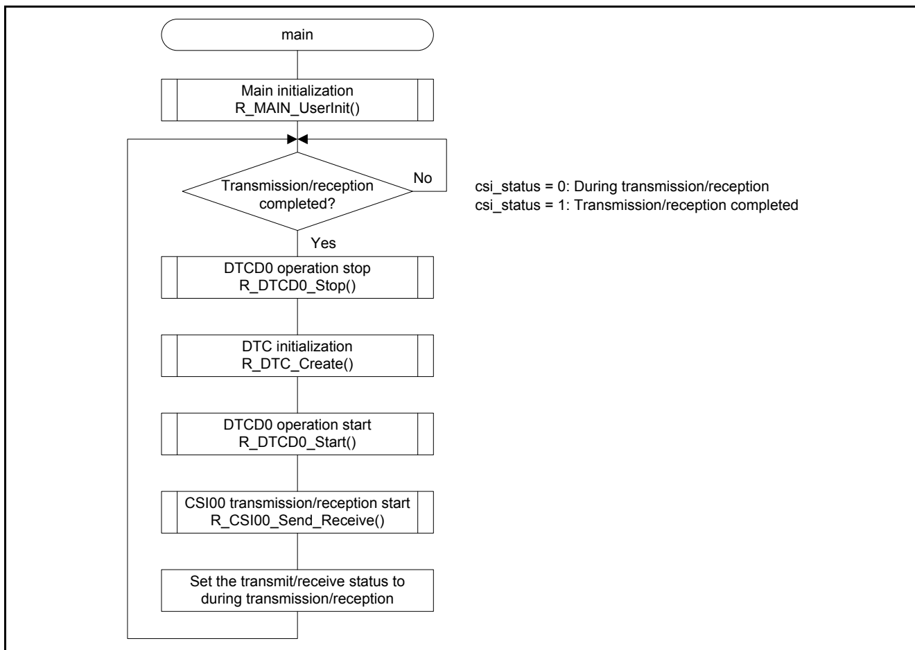
Figure 4.19 Main Processing
