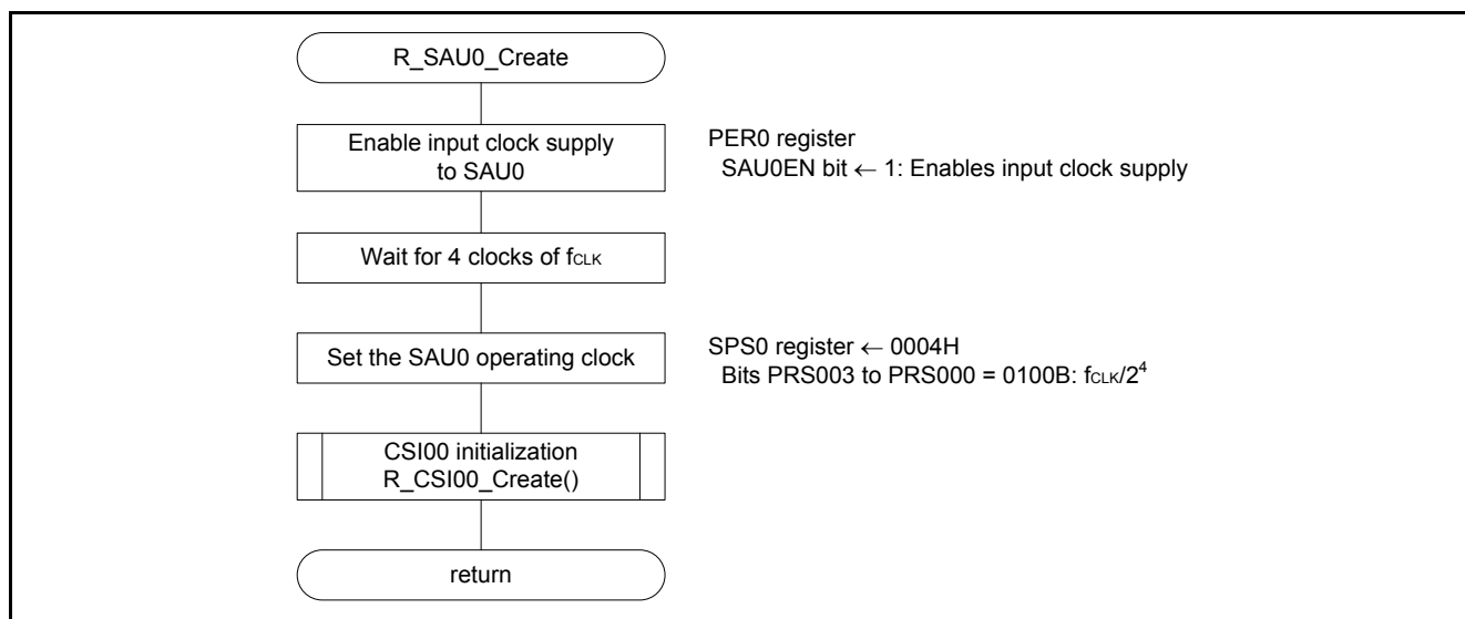
Figure 4.9 SAU0 Initialization
