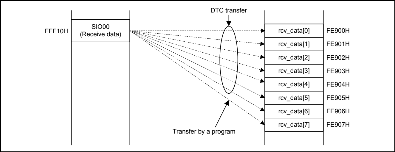
Figure 4.3 DTCD0 Operation
