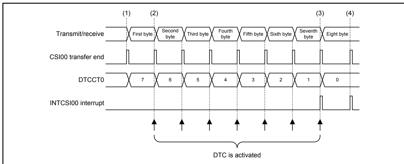
Figure 4.2 Timing of Transmission/Reception and DTC Activation
