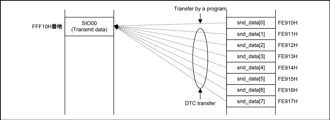
Figure 4.4 DTCD1 Operation
