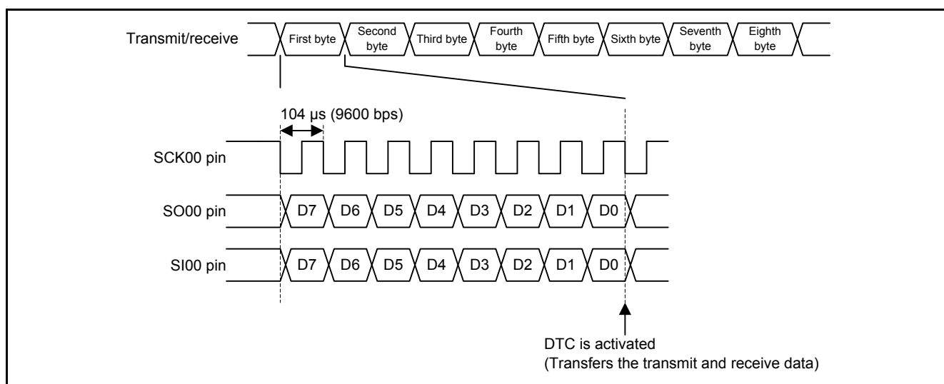
Figure 1.1 Timing and Communication Format
