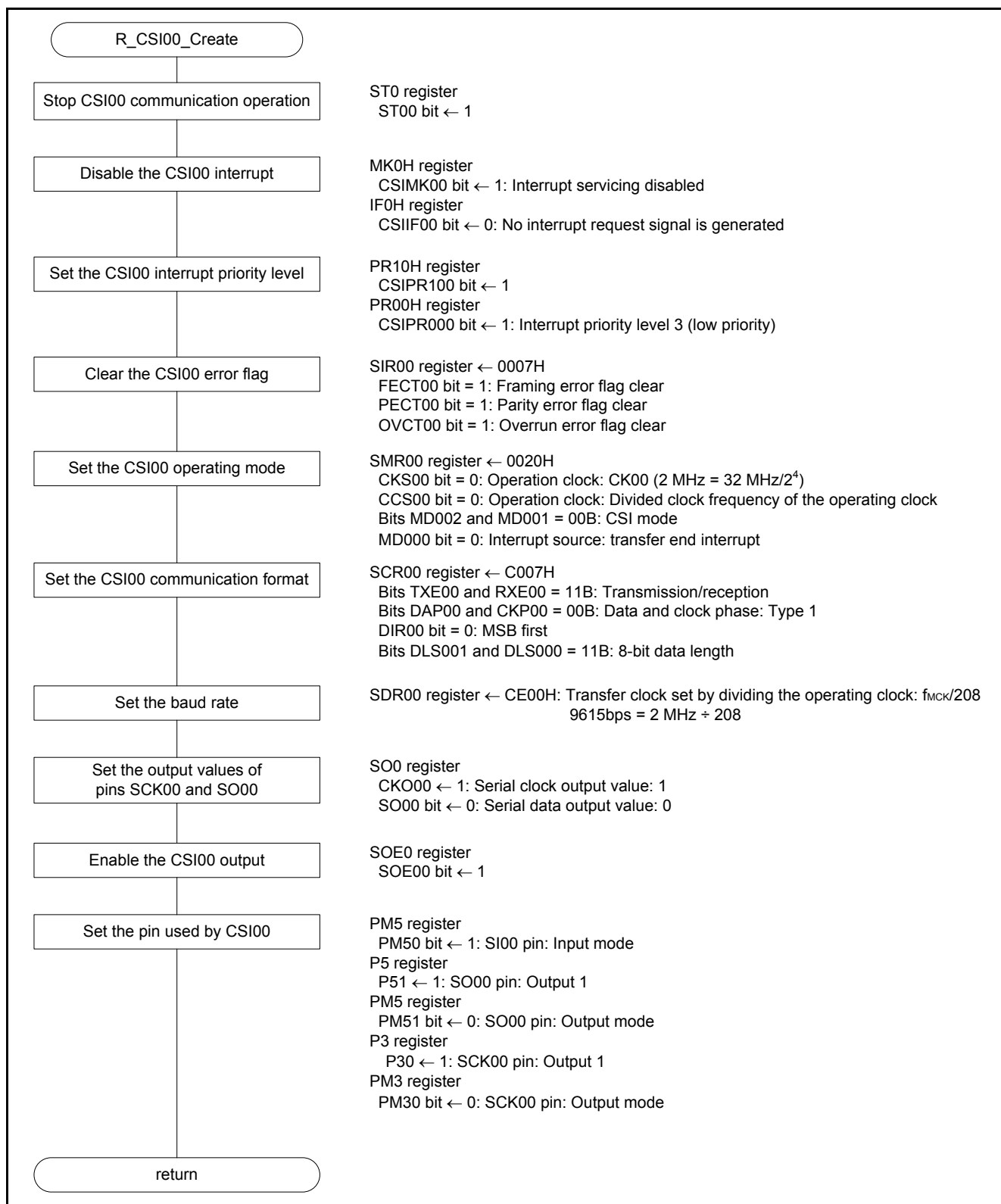
Figure 4.10 CSI00 Initialization
