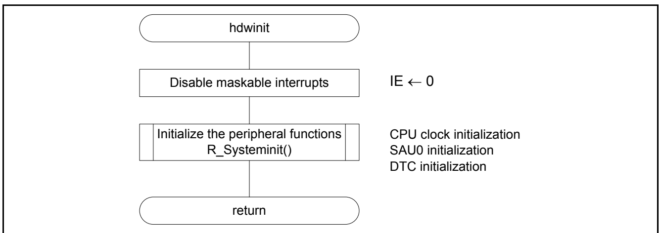
Figure 4.6 Initialization
