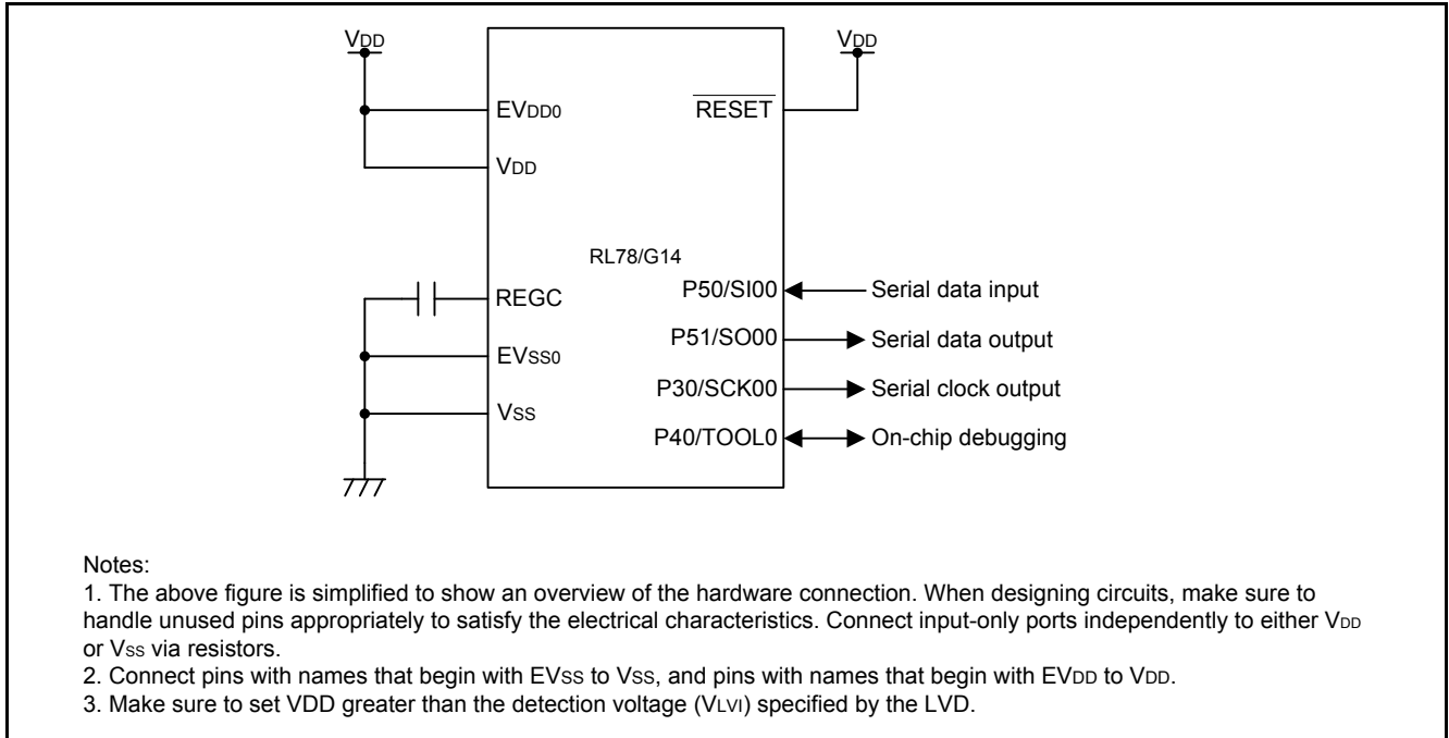
Figure 3.1 Connection Example
