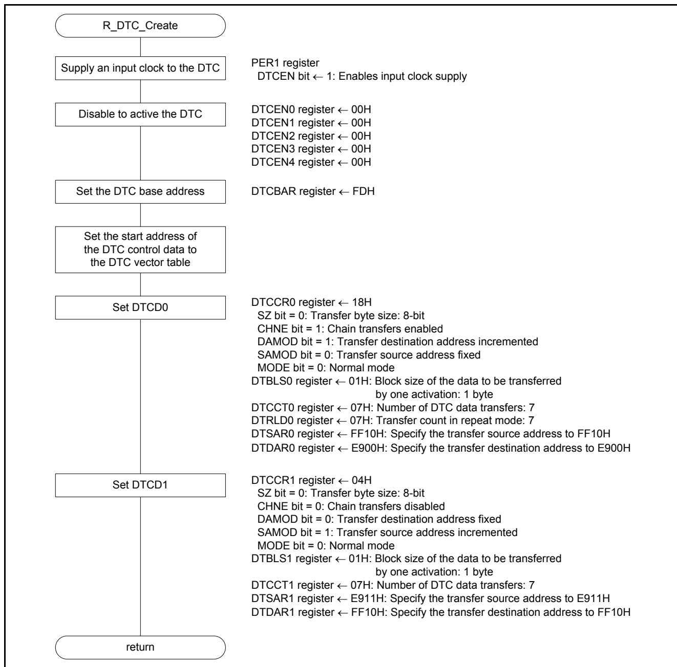
Figure 4.16 DTC Initialization
