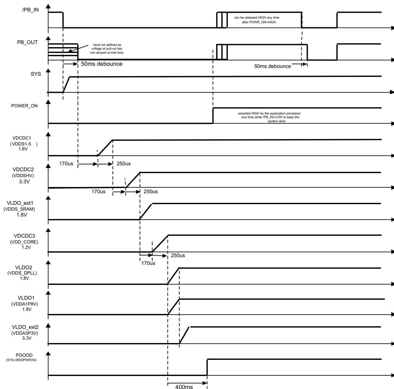
Figure 61. Sequence Using TPS650732 for AM3505
