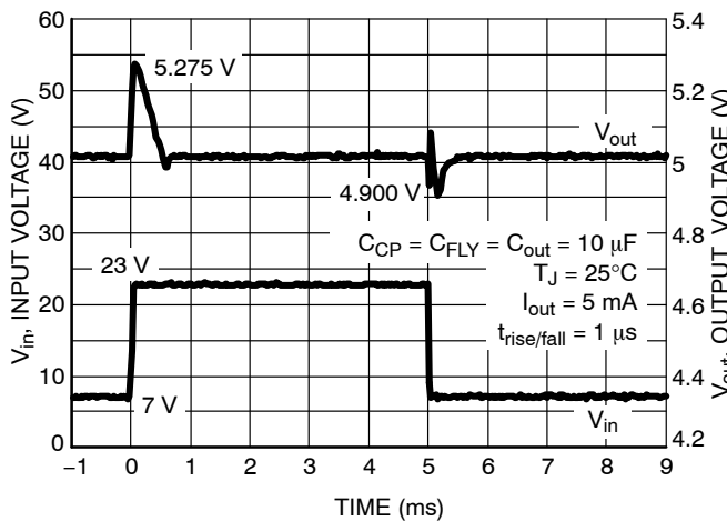
Figure 14. Line Transient
