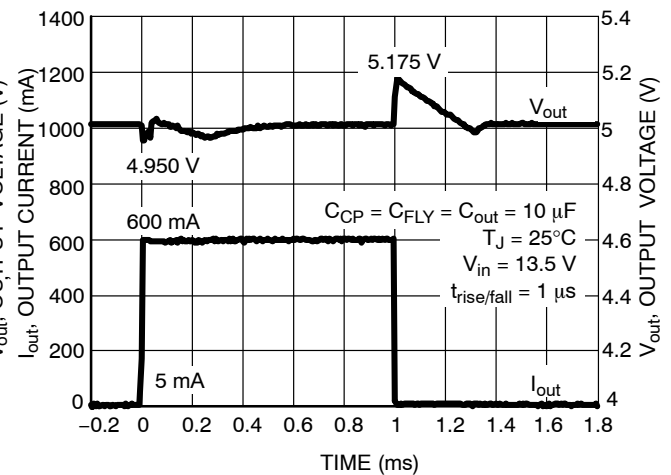
Figure 15. Load Transient
