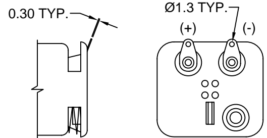
PDSN-38-2C SOLDER LUGS
