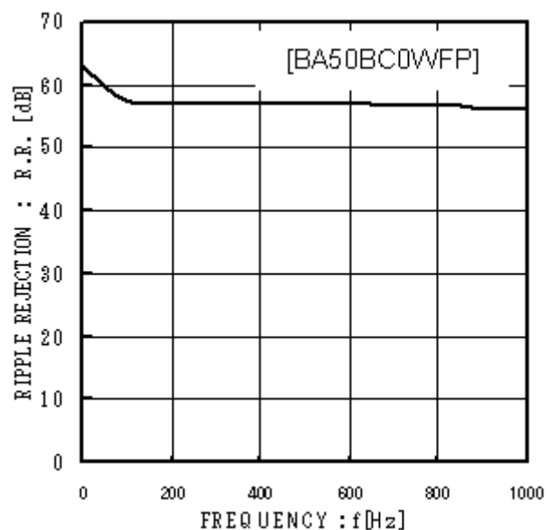
Fig.9 Ripple Rejection
