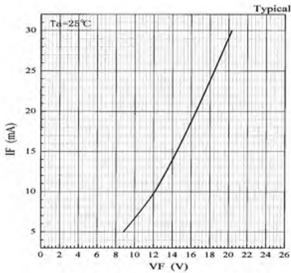
Fig. 1 Forward characteristic [VF-IF]
