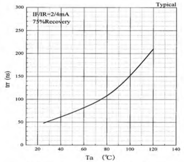
Fig. 4 Reverse recovery time characteristic [Ta-trr]
