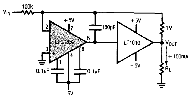
± 100mA Output Drive
