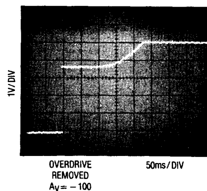
Overload Recovery (Output Clamp Not Used)
