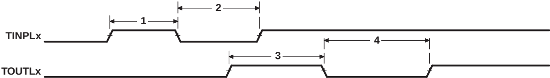
Figure 7-73. Timer Timing
