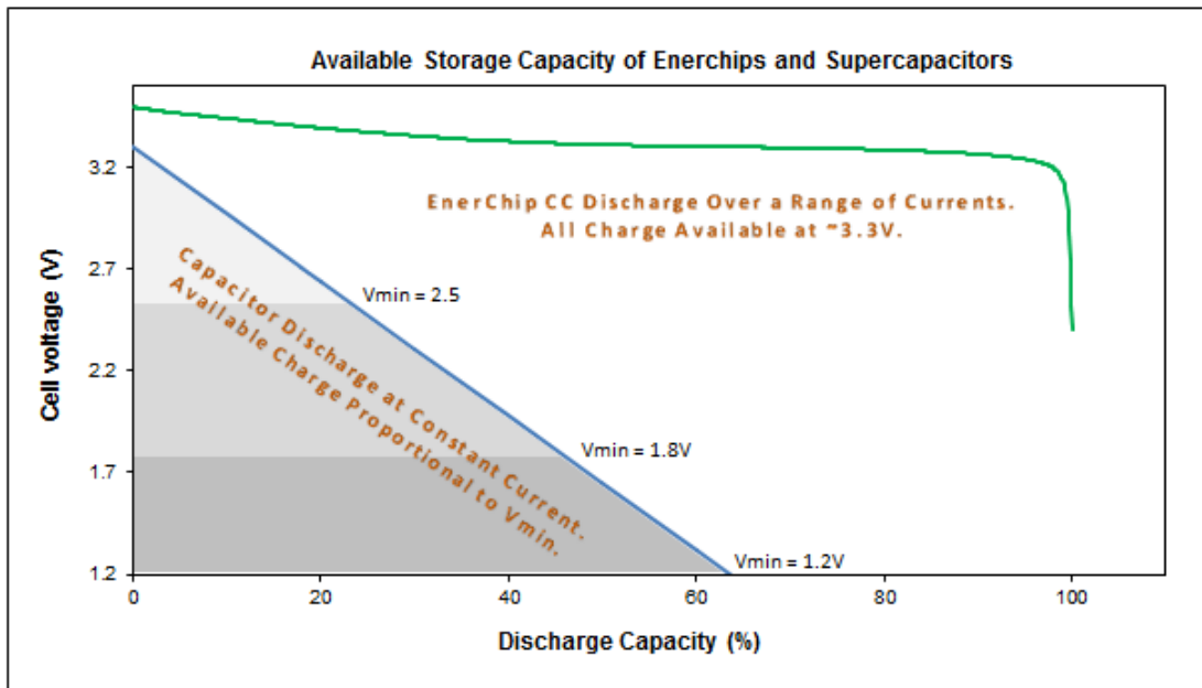
Figure 1: Relative Charge Capacity Delivered to a Load - Green Line Represents the EnerChip CC; Blue Line Represents a Supercapacitor.
