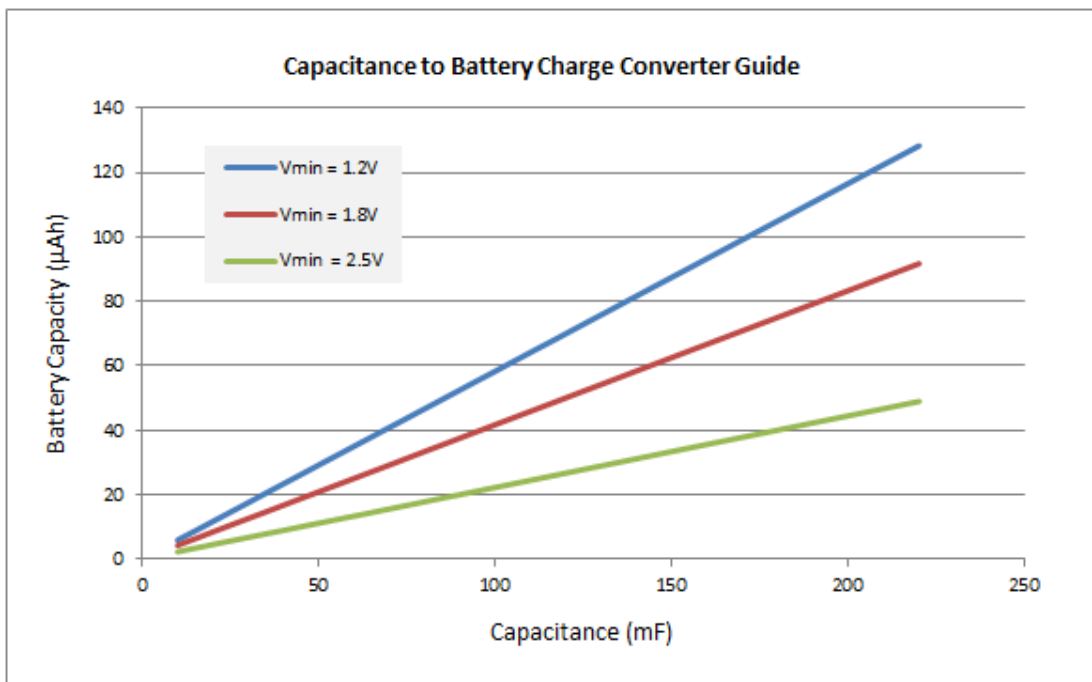
Figure 2: Charge Capacity of EnerChips vs. Supercapacitors at Several Discharge Cutoff Voltage Levels.
