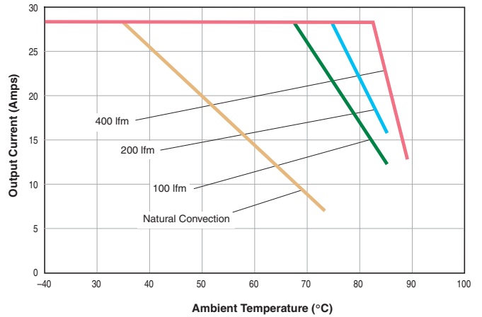
LEN-1.8/28-D12 Maximum Current Temperature Derating VIN = 12V (without heatsink)
