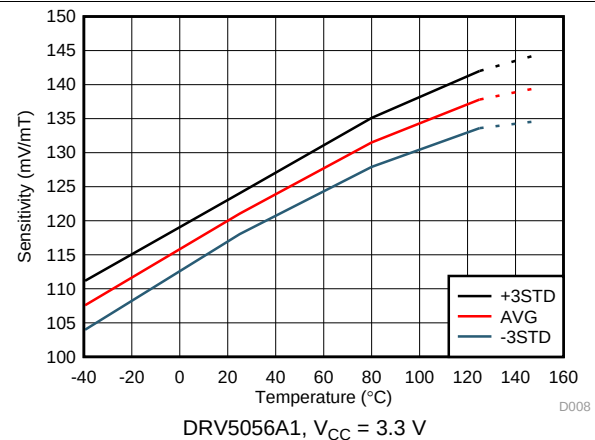
Figure 6. Sensitivity vs Temperature
