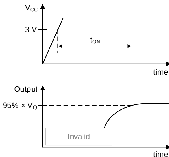
Figure 19. t_{ON} Definition
