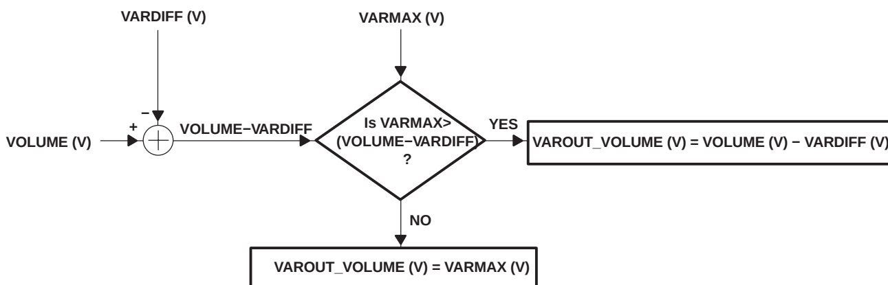
Figure 35. Block Diagram of VAROUT Volume Control
