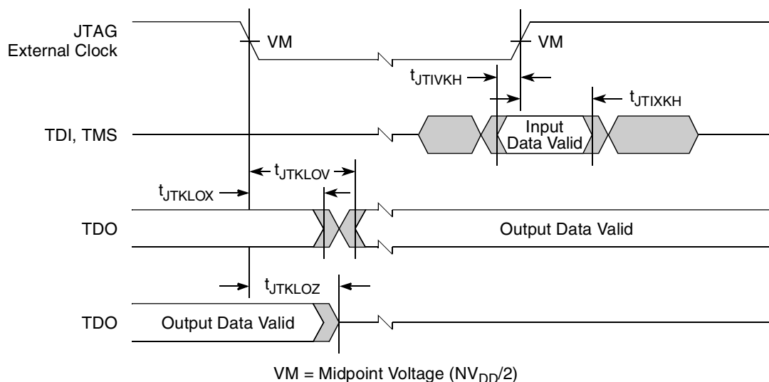
Figure 30. Test Access Port Timing Diagram
