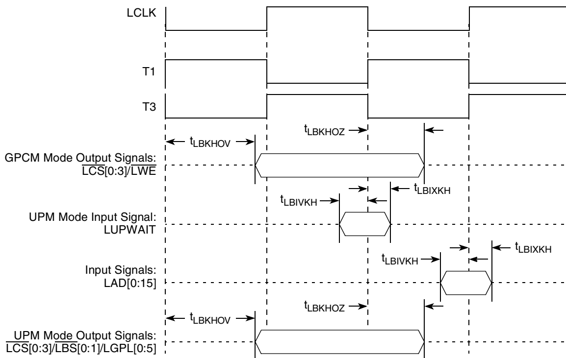
Figure 23. Local Bus Signals, GPCM/UPM Signals for LCCR[CLKDIV] = 2
