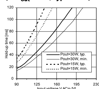
Hold-up time with ACin (at V_{out} = 10\text{V} , typ. + min.)
