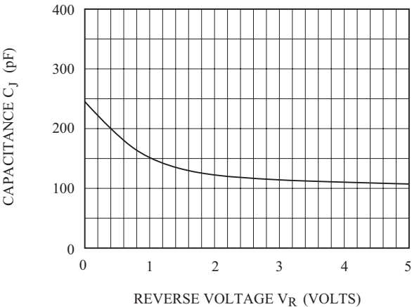
C_J - V_R
