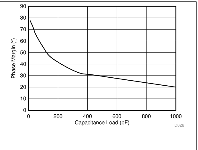
Figure 26. Phase Margin vs Capacitive Load
