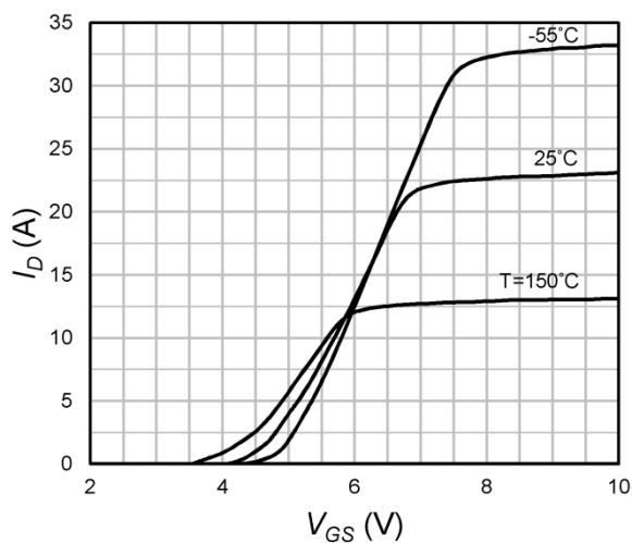
Fig.5 Transfer Characteristics
