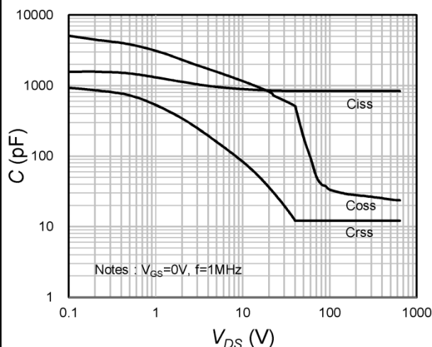
Fig.8 Capacitance Characteristics
