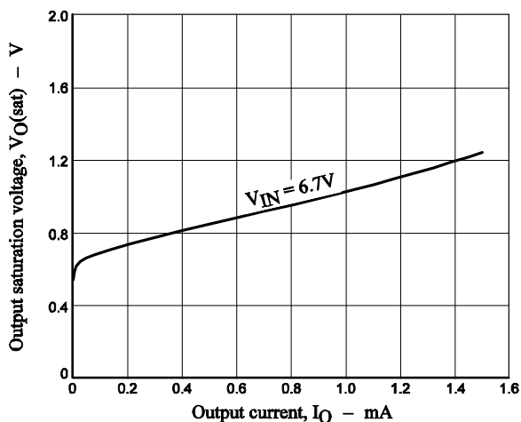
Figure 8. V_{O(sat)} - I_O
