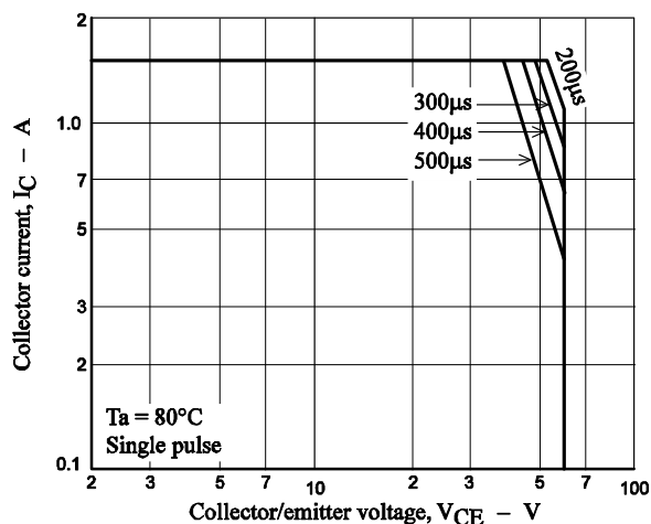
Figure 9. ASO
