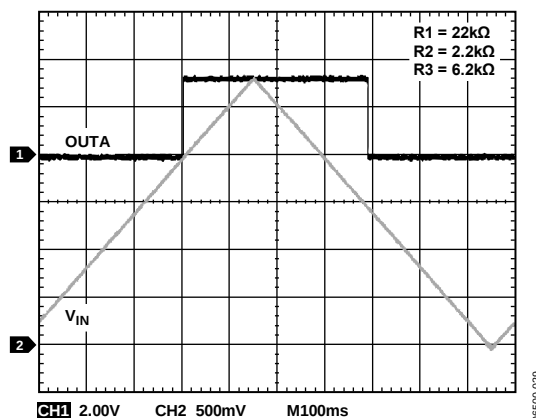
Figure 3. Hysteresis programmed to 513 mV @ V_{IN} on ADCMP341
