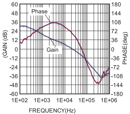
Bode Plot
