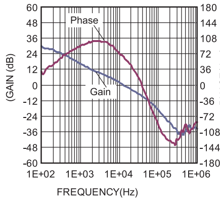
Bode Plot
