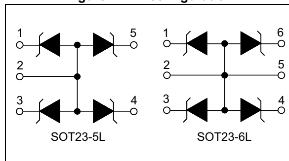
Figure 1. Pin configuration
