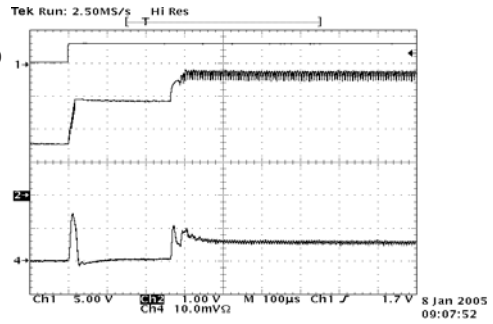
Startup 700mA Flash, Vin = 3.6V, Vout = 3.65V
