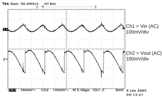
Ripple 200mA Torch, Vin = 3.6V, Vout = 3.9V
