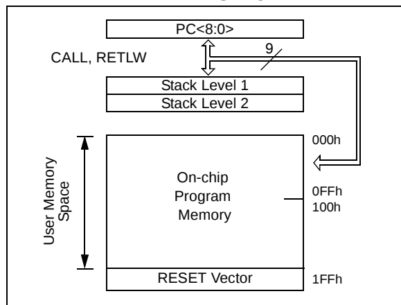
FIGURE 6-1: PIC16C54/CR54/C55 PROGRAM MEMORY MAP AND STACK
