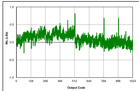
FIGURE 36-66: ADC 10-bit Mode, Single-Ended INL, V_{DD} = 3.0V , T_{AD} = 4\text{ }\mu\text{S} , 25^\circ\text{C} .
