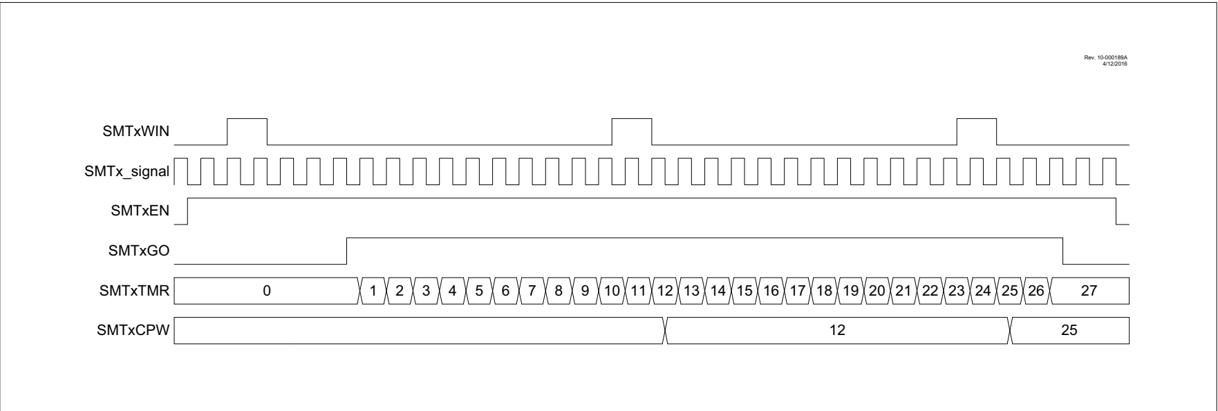
FIGURE 29-18: COUNTER MODE TIMING DIAGRAM
