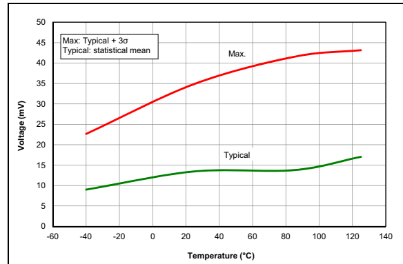
FIGURE 36-54: LPBOR Reset Hysteresis.
