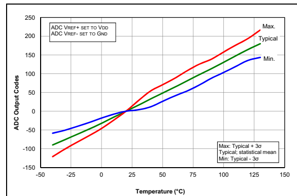
FIGURE 36-77: Temp. Indicator Slope Normalized to 20^\circ C , Low Range, V_{DD} = 1.8V , PIC16LF1614/8 Only.
