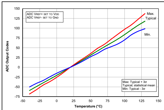
FIGURE 36-74: Temp. Indicator Slope Normalized to 20^\circ C , High Range, V_{DD} = 5.5V , PIC16F1614/8 Only.
