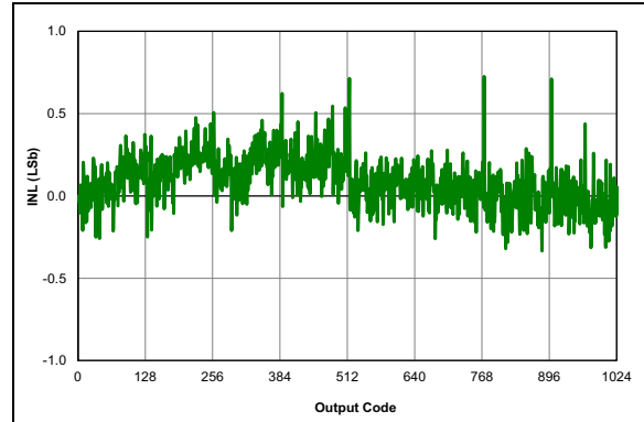
FIGURE 36-65: ADC 10-bit Mode, Single-Ended INL, V_{DD} = 3.0V , T_{AD} = 1\text{ }\mu\text{S} , 25^\circ\text{C} .
