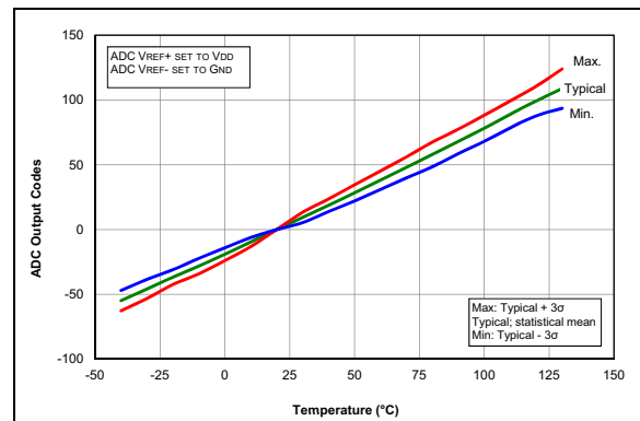
FIGURE 36-78: Temp. Indicator Slope Normalized to 20^\circ C , Low Range, V_{DD} = 3.0V , PIC16LF1614/8 Only.
