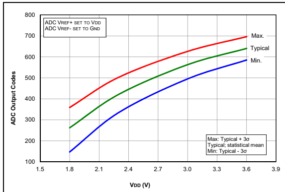
FIGURE 36-73: Temp. Indicator Initial Offset, Low Range, Temp. = 20^\circ C , PIC16LF1614/8 Only.
