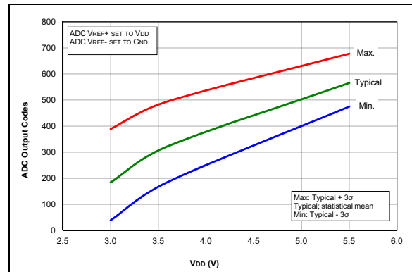
FIGURE 36-71: Temp. Indicator Initial Offset, High Range, Temp. = 20^\circ\text{C} , PIC16F1614/8 Only.
