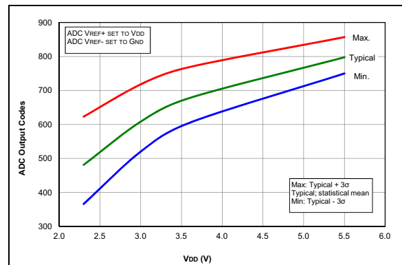
FIGURE 36-72: Temp. Indicator Initial Offset, Low Range, Temp. = 20^\circ\text{C} , PIC16F1614/8 Only.
