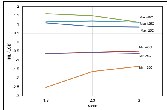
FIGURE 36-70: ADC 10-bit Mode, Single-Ended INL, V_{DD} = 3.0V , T_{AD} = 1\text{ }\mu\text{s} .
