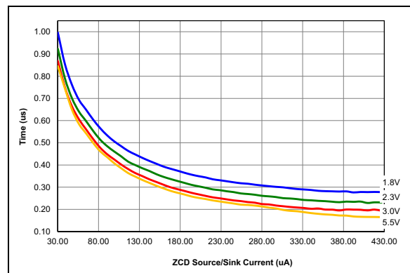
FIGURE 36-102: ZCD Pin Response Timer over Current, Typical Measured Values from -40^\circ C to 125^\circ C .
