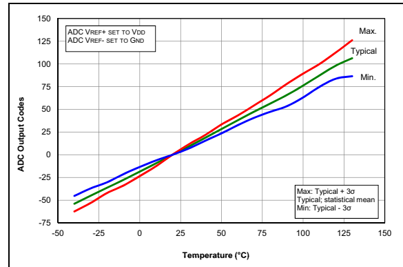
FIGURE 36-76: Temp. Indicator Slope Normalized to 20^\circ C , Low Range, V_{DD} = 3.0V , PIC16F1614/8 Only.
