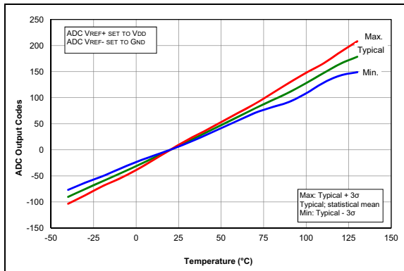
FIGURE 36-75: Temp. Indicator Slope Normalized to 20^\circ C , High Range, V_{DD} = 3.0V , PIC16F1614/8 Only.
