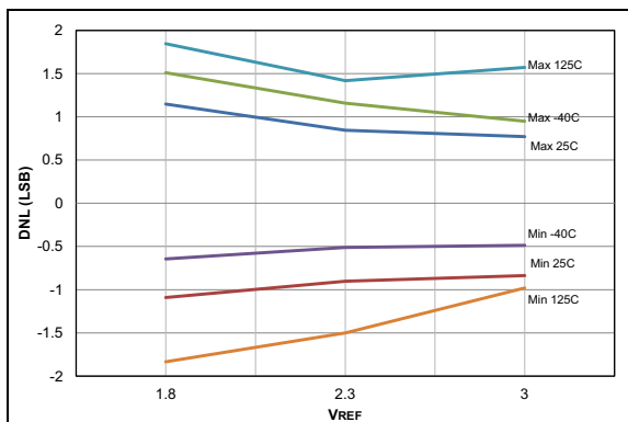
FIGURE 36-69: ADC 10-bit Mode, Single-Ended DNL, V_{DD} = 3.0V , T_{AD} = 1\text{ }\mu\text{s} .
