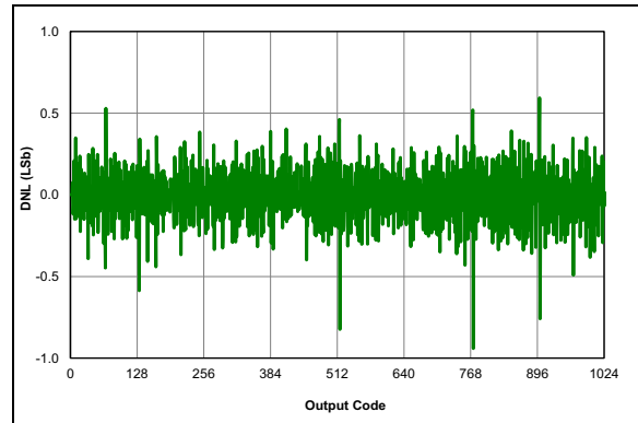
FIGURE 36-64: ADC 10-bit Mode, Single-Ended DNL, V_{DD} = 3.0V , T_{AD} = 4\text{ }\mu\text{S} , 25^\circ\text{C} .
