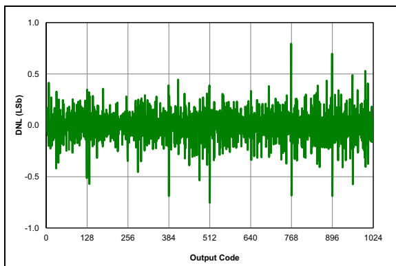
FIGURE 36-63: ADC 10-bit Mode, Single-Ended DNL, V_{DD} = 3.0V , T_{AD} = 1\text{ }\mu\text{S} , 25^\circ\text{C} .
