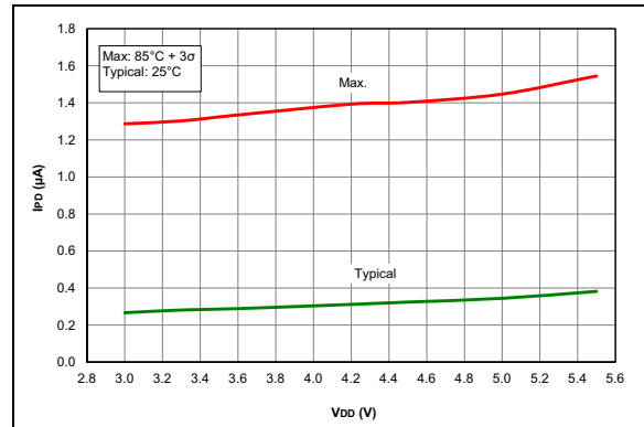
FIGURE 36-28: I_{PD} , LP Brown-Out Reset (LPBOR = 0), PIC16F1614/8 Only.
