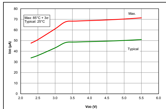
FIGURE 36-12: I_{DD} Maximum, EC Oscillator HP Mode, PIC16F1614/8 Only.
