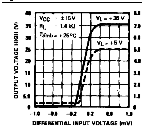
Figure 12. Transfer function
