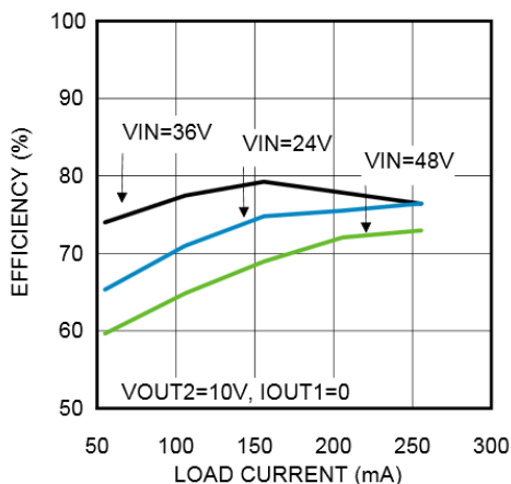
Figure 21. Efficiency at 750 kHz, V_{OUT1} = 10 V
