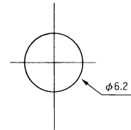
Recommended Panel Mounting Hole
