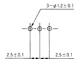
Recommended PCB Mounting Holes
