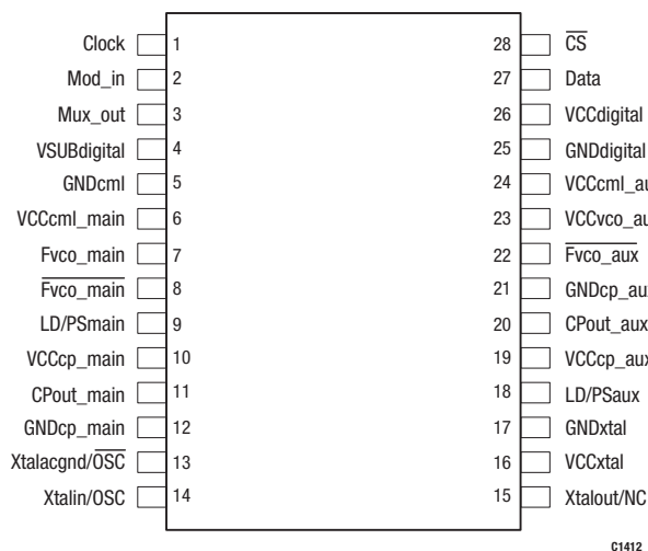
Figure 2. SKY72300-21 Pinout, 28-Pin EP-TSSOP (Top View)
