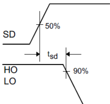
Figure 3. Shutdown Waveform Definitions
