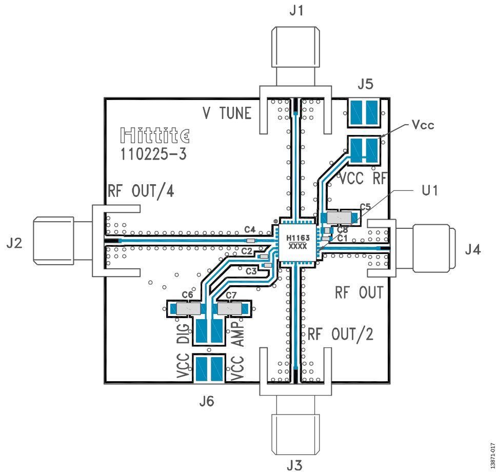
Figure 17. Evaluation PCB
