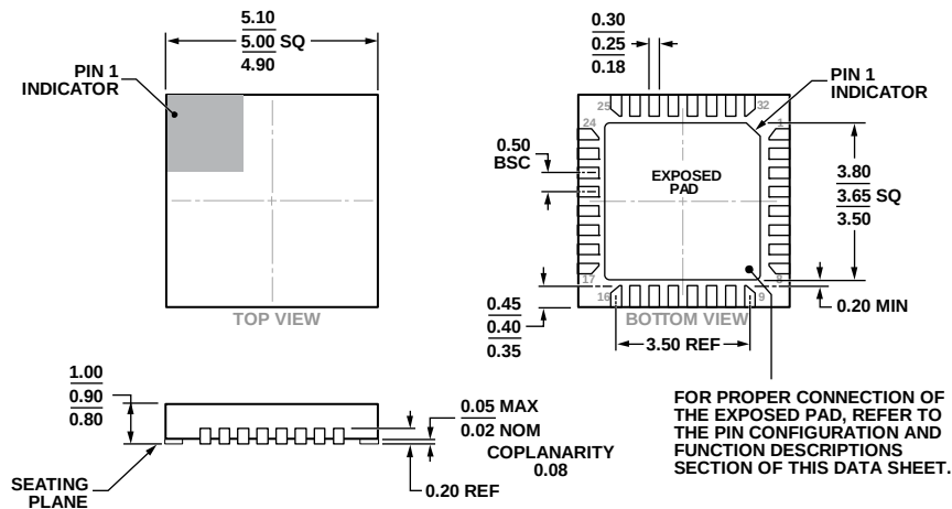
Figure 18. 32-Lead Lead Frame Chip Scale Package [LFCSP] 5 mm x 5 mm Body and 0.90 mm Package Height (HCP-32-1) Dimensions shown in millimeters
