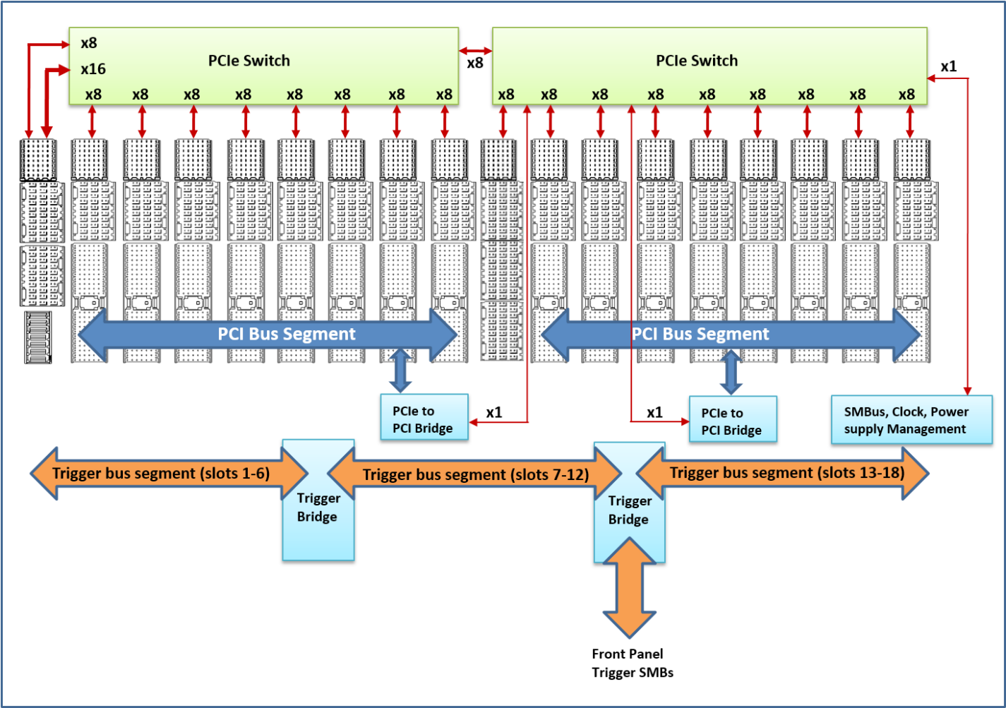
Figure 3. Backplane configuration diagram of the M9019A PXIe 18-slot chassis.
