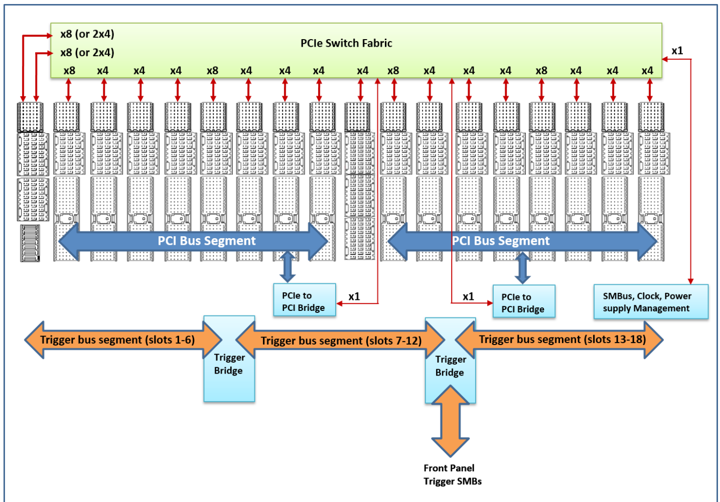
Figure 2. Backplane configuration diagram of the M9018B PXIe 18-slot chassis.
