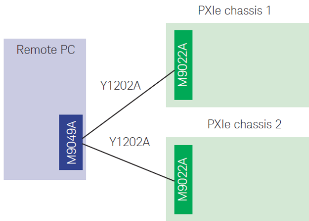
Figure 8. Star configuration using the M9049A for x8 connections from a remote PC to two chassis. Chassis types can be mixed AXIe and PXIe
