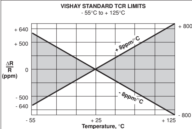
FIGURE 3 - TEMPERATURE COEFFICIENT OF RESISTANCE CURVE ( 55^\circ\text{C} TO +125^\circ\text{C} )
