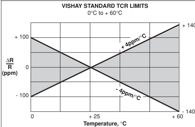
FIGURE 2 - TEMPERATURE COEFFICIENT OF RESISTANCE CURVE ( 0^\circ\text{C} TO +60^\circ\text{C} )
