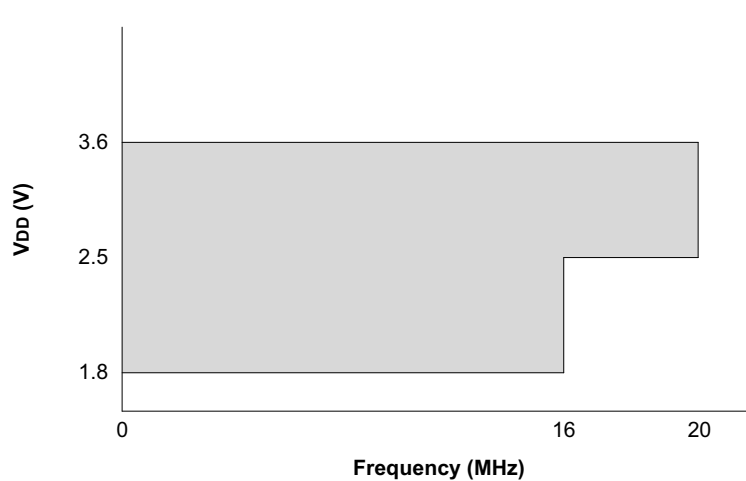
FIGURE 25-2: VOLTAGE FREQUENCY GRAPH, -40^{\circ}\text{C} \leq T_A \leq +125^{\circ}\text{C} , PIC16LF1507 ONLY
