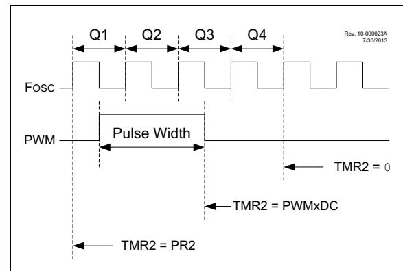
FIGURE 19-2: PWM OUTPUT
