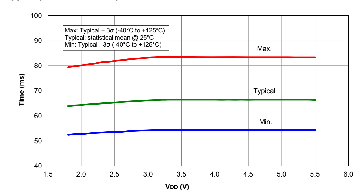
FIGURE 26-47: PWRT PERIOD
