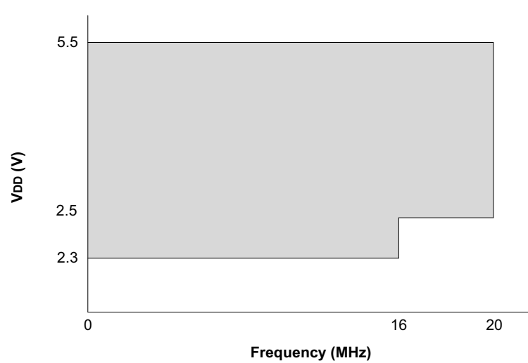
FIGURE 25-1: VOLTAGE FREQUENCY GRAPH, -40^{\circ}\text{C} \leq T_A \leq +125^{\circ}\text{C} , PIC16F1507 ONLY
