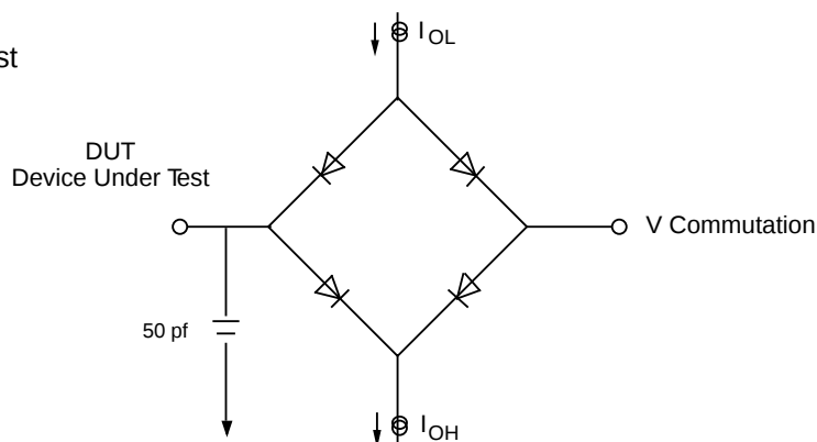
Test Load Diagram
