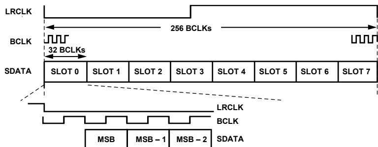
Figure 61. TDM 8 Mode
