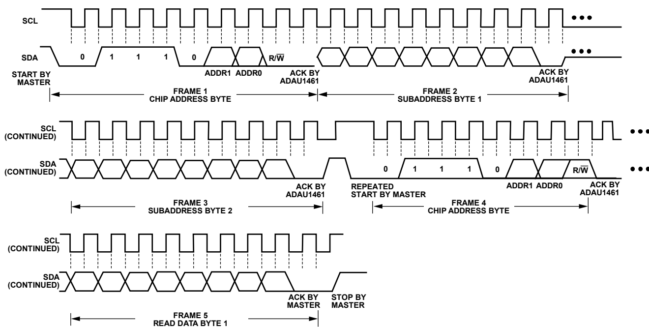
Figure 50. I 2 C Read from ADAU1461 Clcking
