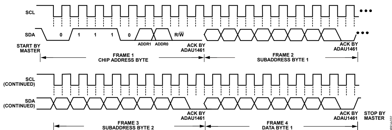
Figure 49. I 2 C Write to ADAU1461 Clcking
