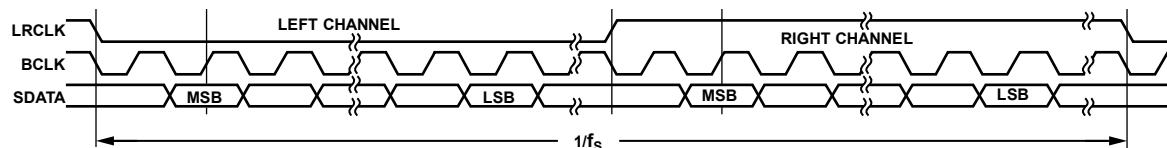
Figure 58. I²S Mode—16 Bits to 24 Bits per Channel
